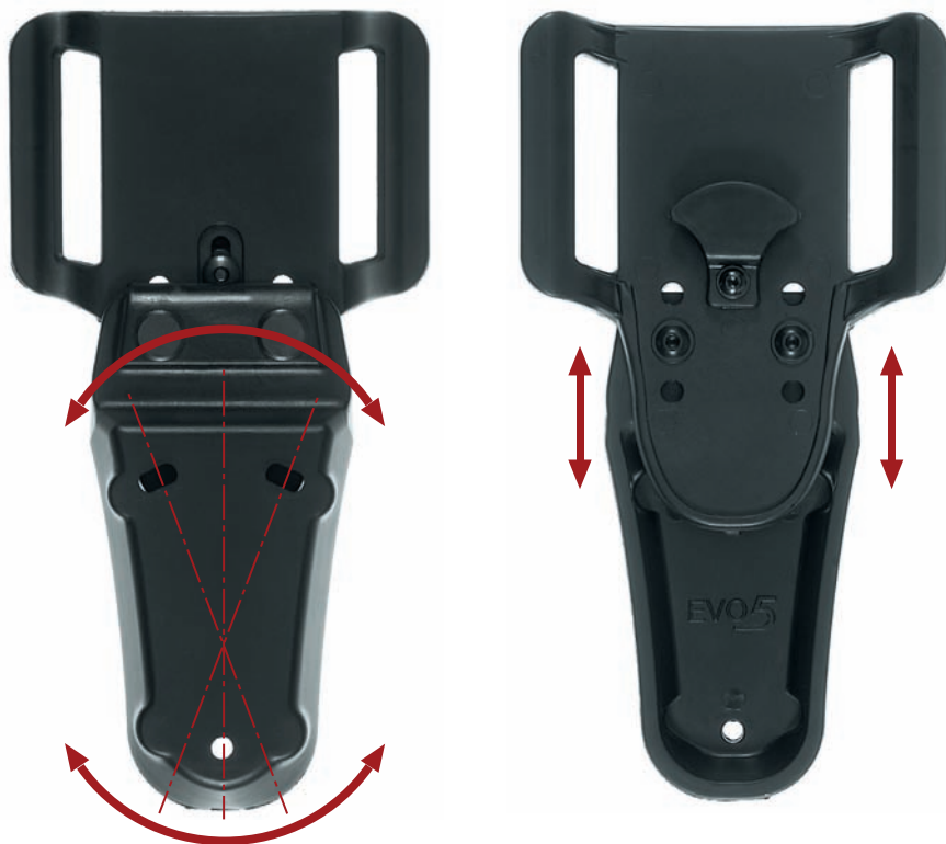
55850 BLE Belt Loop in polymer. Realised in two parts. Assembled with 3 screws. Adjustable in height with 3 different positions. Adjustable inclination. Belt stopper, that does not allow movement of the holster on the belt.
