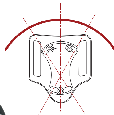
BLA Belt loop in polymer, HIGH position, MULTI position
